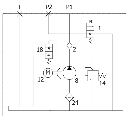
Hydraulic Schematic
